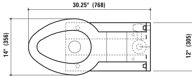
FIXTURE PLAN VIEW
