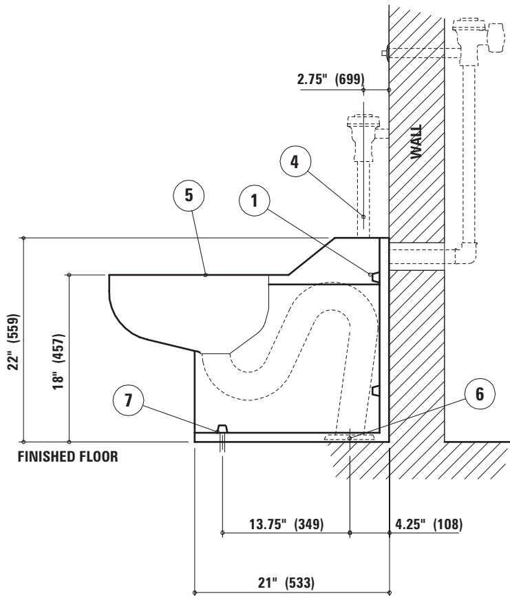
WALL ELEVATION VIEW (fixture side)
