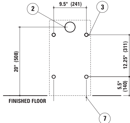
WALL ELEVATION VIEW (fixture side)
