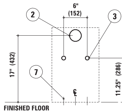
WALL ELEVATION VIEW (fixture side)
