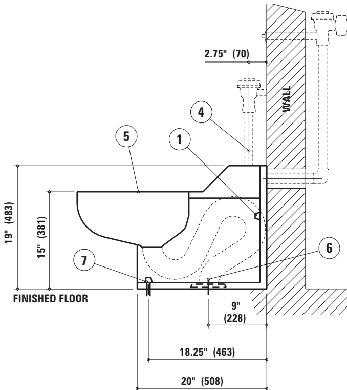
FIXTURE SIDE VIEW
