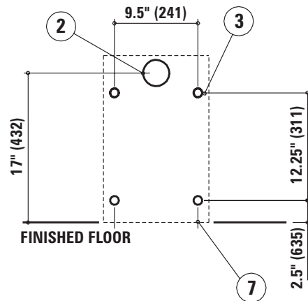
WALL ELEVATION VIEW (fixture side)
