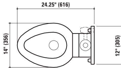
FIXTURE PLAN VIEW
