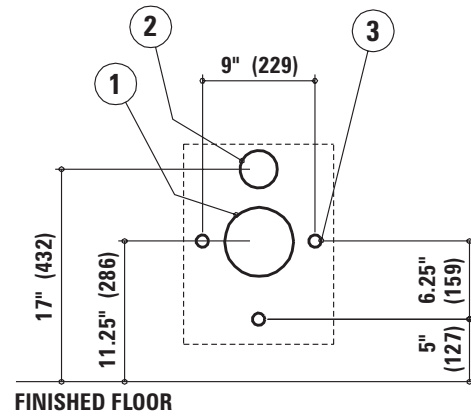
WALL ELEVATION VIEW (fixture side)
