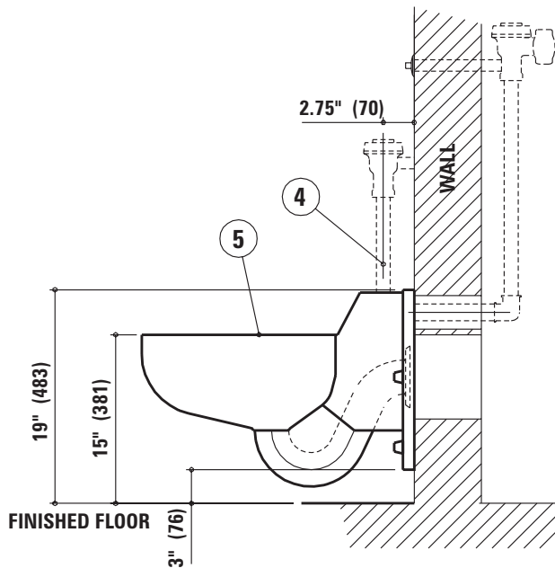
FIXTURE SIDE VIEW
