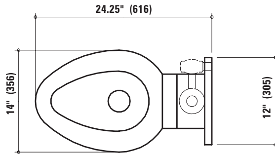
FIXTURE PLAN VIEW
