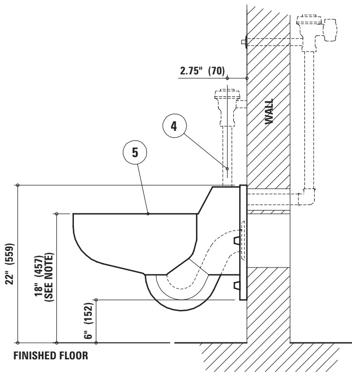
FIXTURE SIDE VIEW
