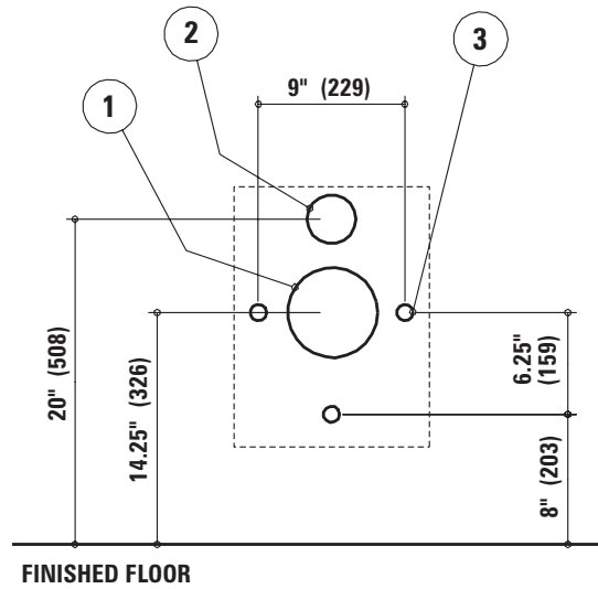
WALL ELEVATION VIEW (fixture side)
