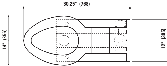
FIXTURE PLAN VIEW
