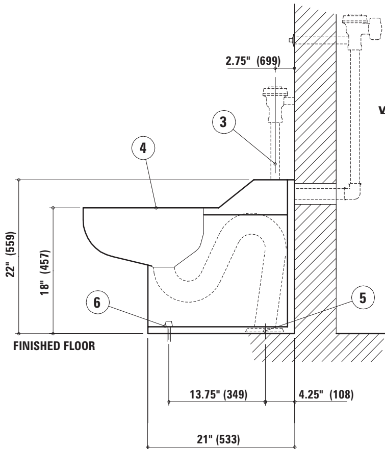
FIXTURE SIDE VIEW
