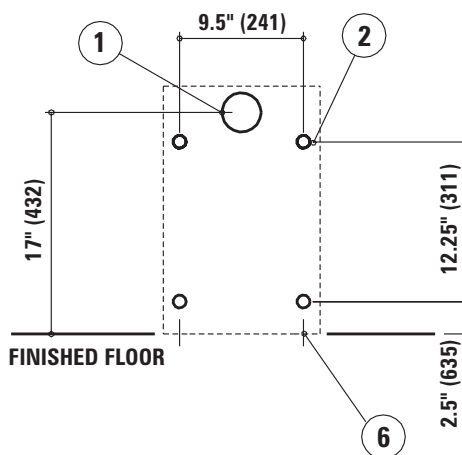
WALL ELEVATION VIEW (fixture side)
