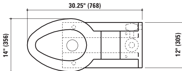
FIXTURE PLAN VIEW
