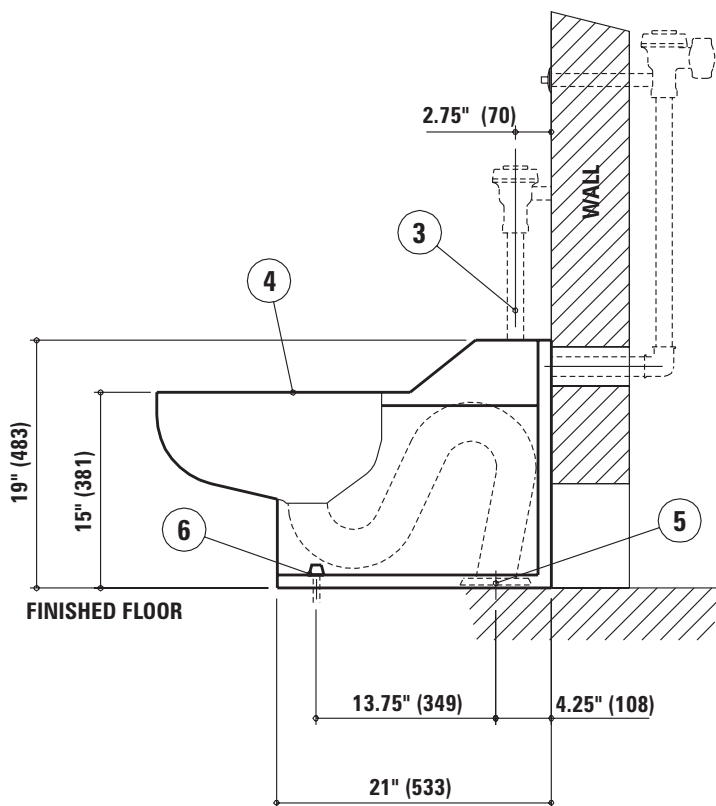
FIXTURE SIDE VIEW
