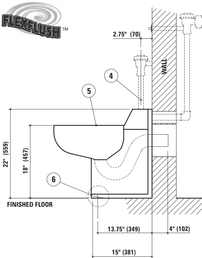
FIXTURE SIDE VIEW
