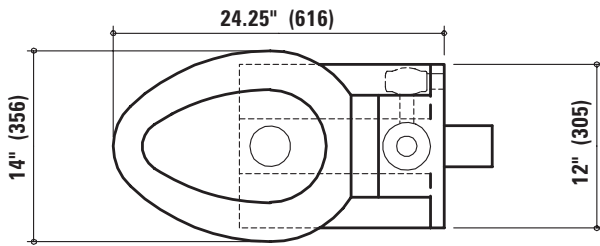
FIXTURE PLAN VIEW
